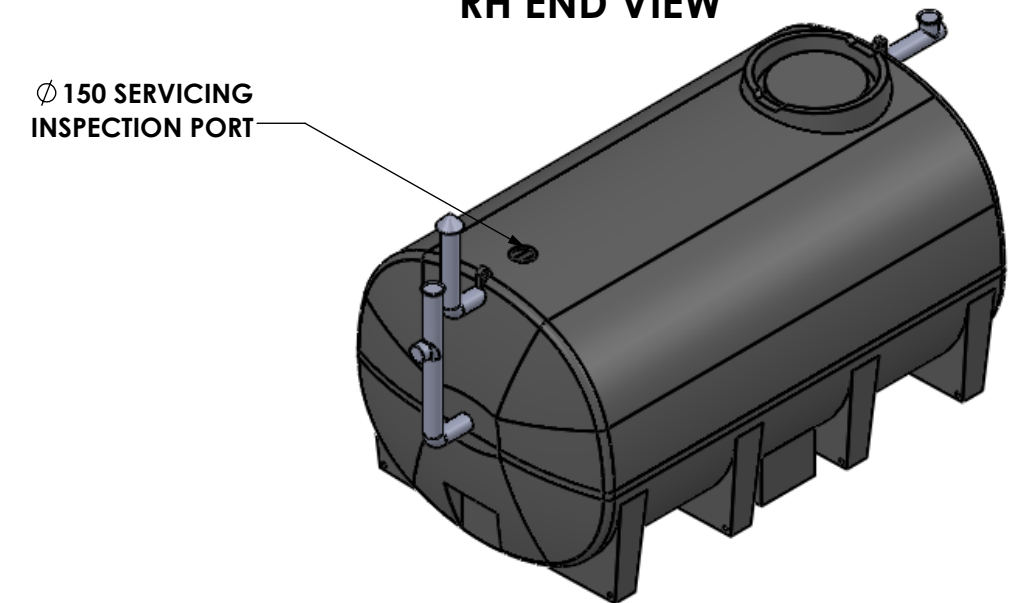
ISOMETRIC VIEW
